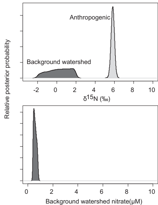
Fig. 3. Parameter estimates for two-source mixing model from Bayesian parameter estimation. Higher posterior densities represent more probable parameter values based on the data. (A) Posterior probability densities for the N isotope value for the background watershed N source and the anthropogenic N source. (B) Posterior probability density of the concentration of nitrate that comes from background watershed sources.
