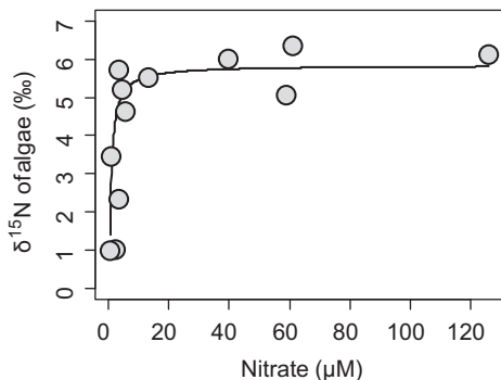
Fig. 2. Observed and predicted N isotopes as a function of stream nitrate. Each open point represents the observed average algal N isotope signature and the corresponding site nitrate concentration. Also shown is the line that represents the best model fit for a two-source mixing model.
